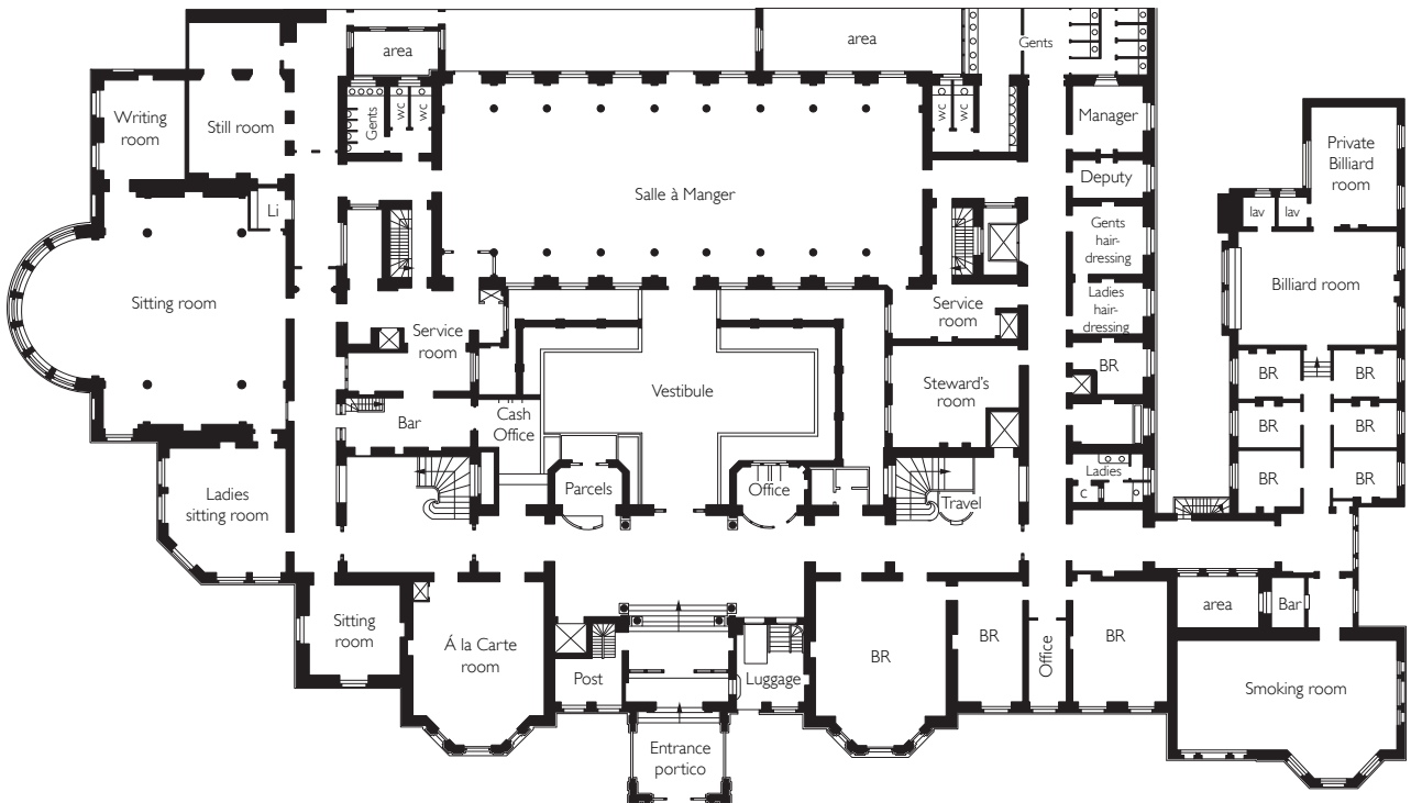
GROUND FLOOR
